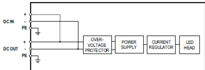
Block diagram
